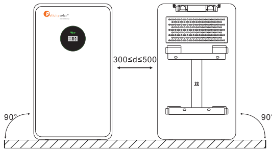
Ground(Two rows installtion)
